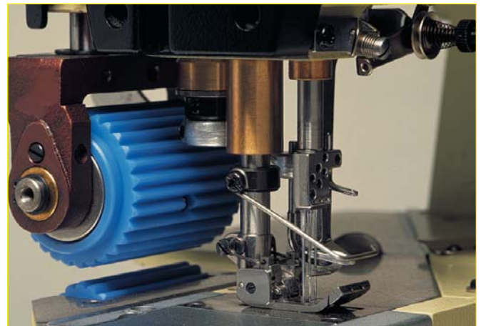
Global® model CB 2723-64 - with puller
